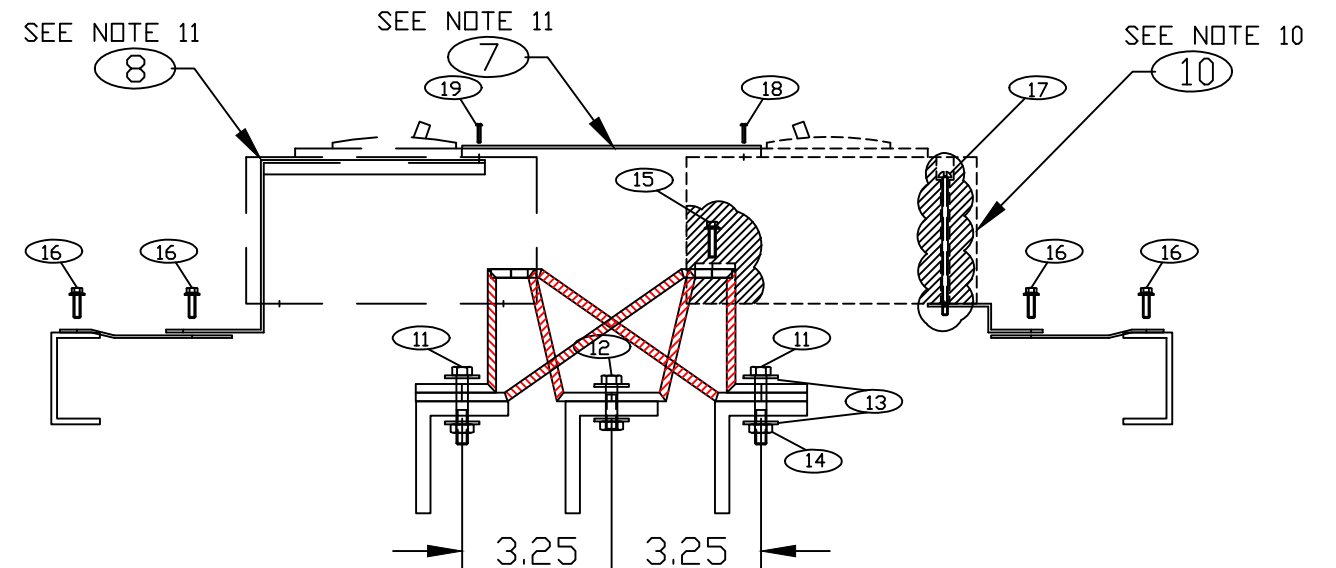
FRONT VIEW SHOWING MOUNTING LOCATIONS OF CONNECTIONS TO BUS BARS AND BREAKER MOUNTING BRACKET TO "Z" RAILS (BREAKER REMOVED TO SHOW CONNECTORS)
