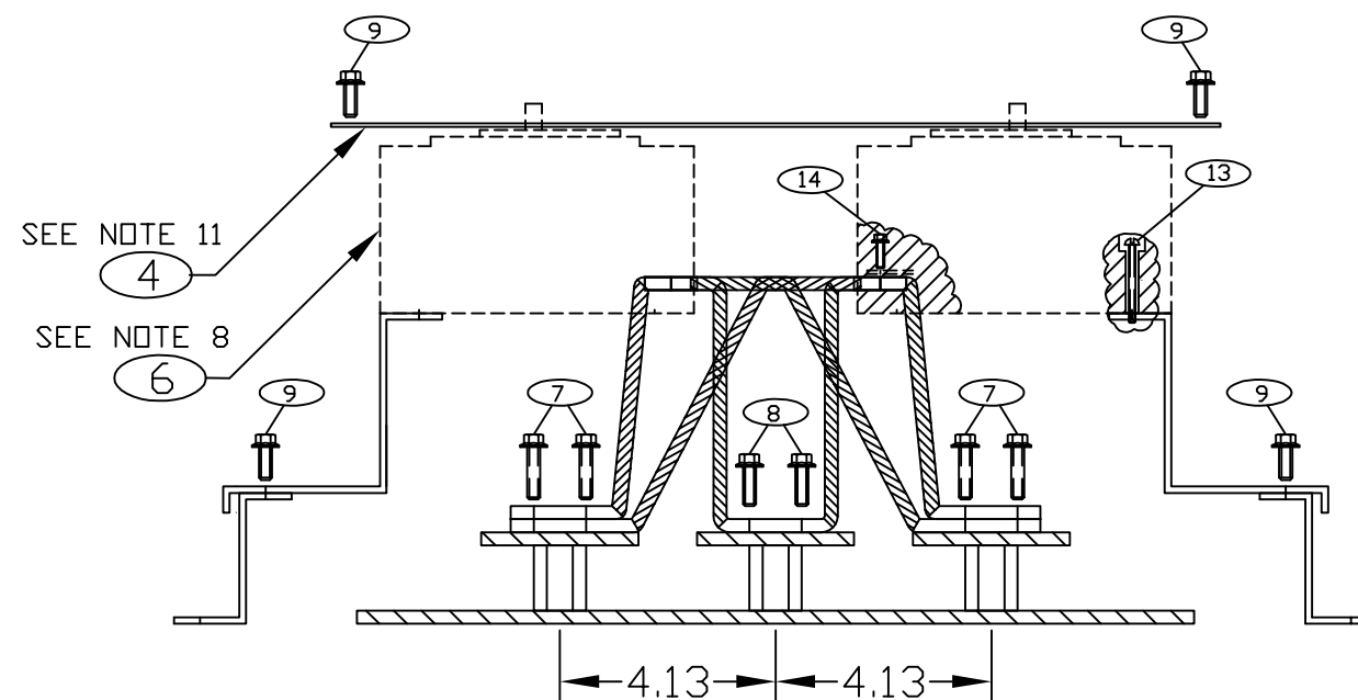
FRONT VIEW SHOWING MOUNTING LOCATIONS OF CONNECTIONS TO BUS BARS AND BREAKER MOUNTING BRACKET TO "Z" RAILS (BREAKER REMOVED TO SHOW CONNECTORS)
