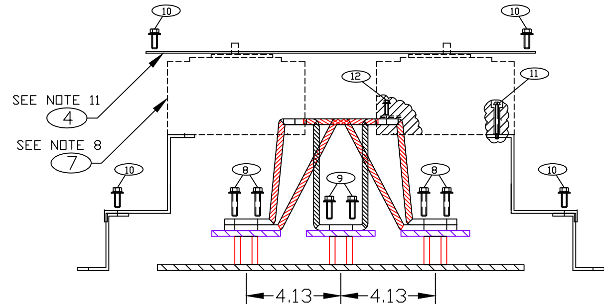
FRONT VIEW SHOWING MOUNTING LOCATIONS OF CONNECTIONS TO BUS BARS AND BREAKER MOUNTING BRACKET TO "Z" RAILS (BREAKER REMOVED TO SHOW CONNECTORS)
