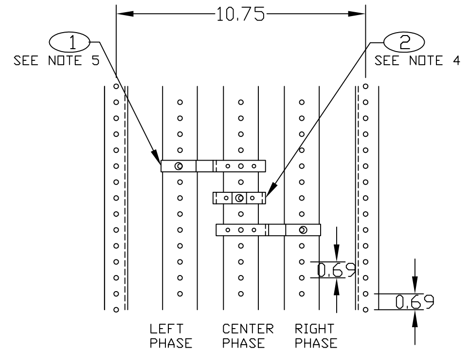
FRONT VIEW SHOWING MOUNTING LOCATIONS OF CONNECTIONS TO BUS BARS AND BREAKER MOUNTING BRACKET TO "Z" RAILS (BREAKER REMOVED TO SHOW CONNECTORS)
